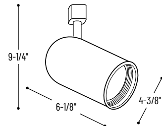
NTH-106B Black Roundback Cylinder with Black Baffle
